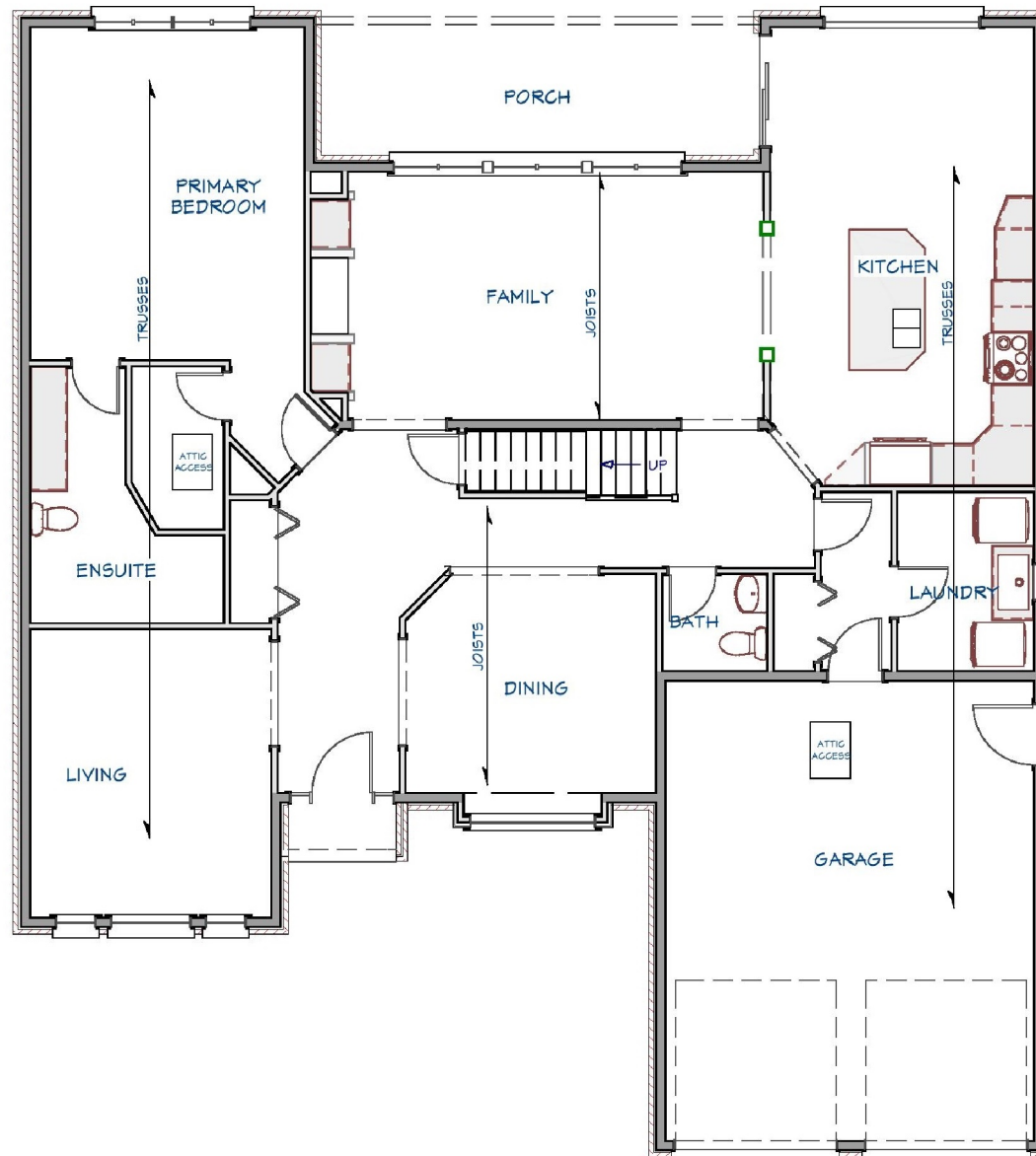
PLAN - AS-BUILT MAIN LEVEL SCALE: N/A
