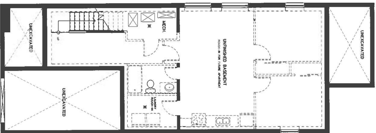
FOUNDATION PLAN
