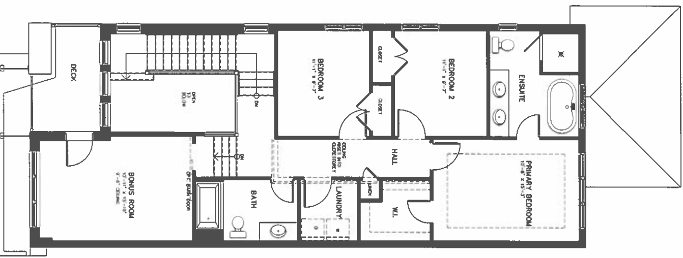
SECOND FLOOR PLAN ELEV. C 1264 SQUARE FEET
